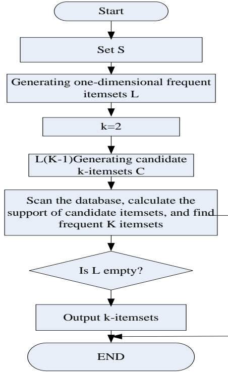
FIGURE 1. Flow chart of fuzzy mathematics trend prediction algorithm
